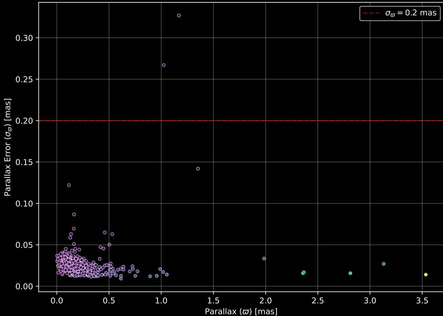
APOGEE DR17 Field: [311-06] Parallax Quality (n= 518)
