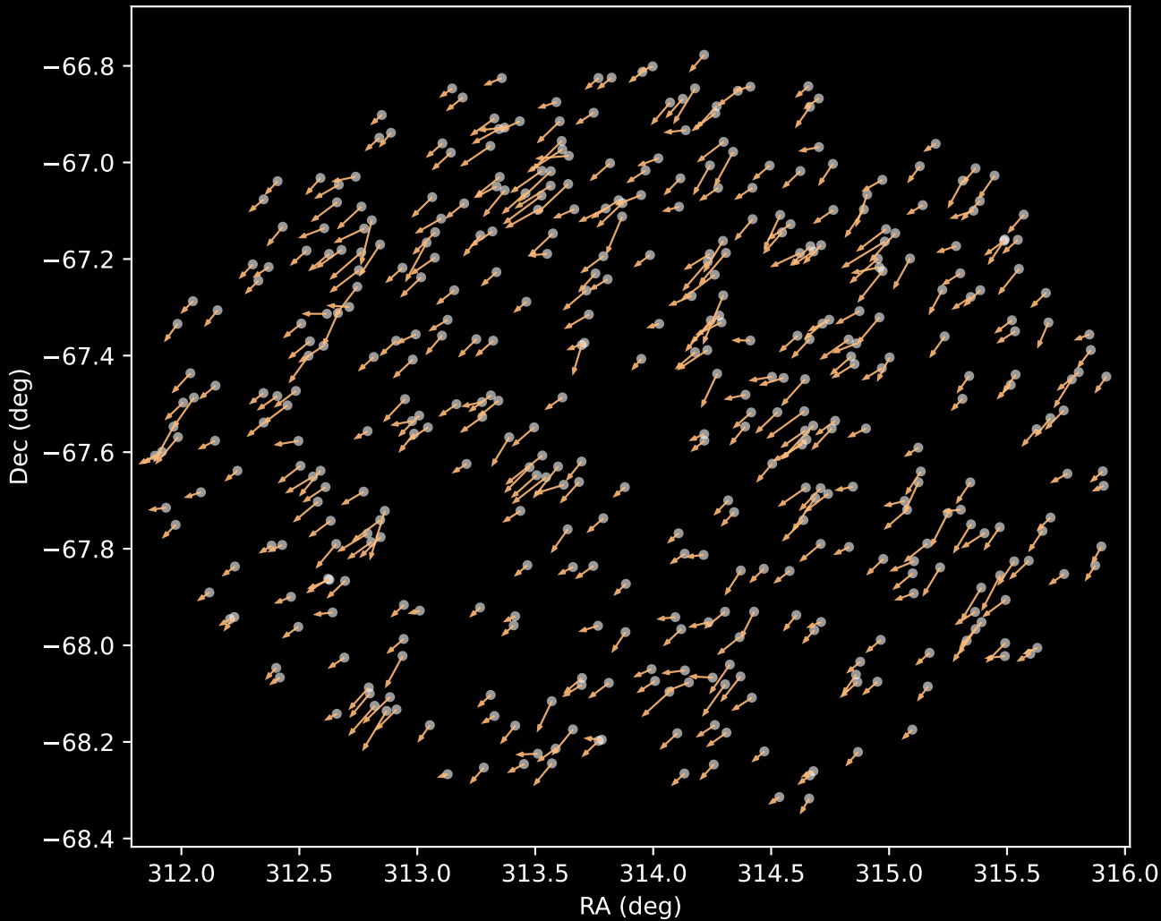
APOGEE DR17 Cluster 3 Proper Motion Vectors (n=430)
