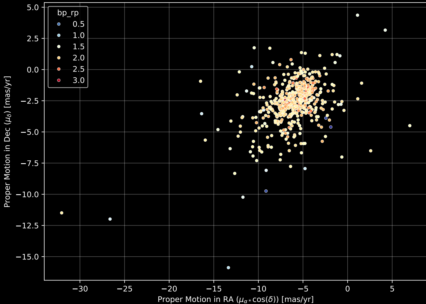
APOGEE DR17 Field: [311-06] Proper Motion Diagram (n= 518)
