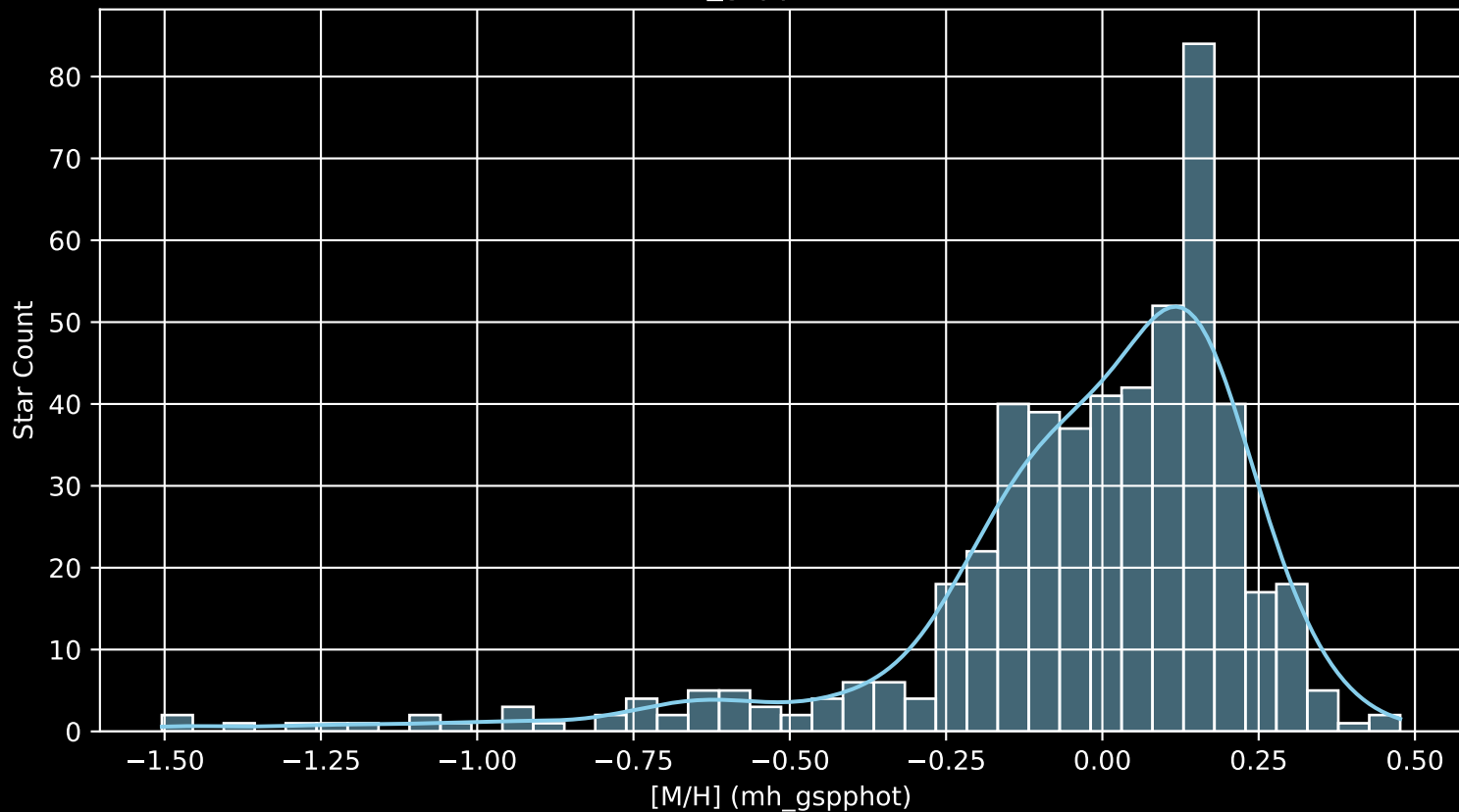
APOGEE DR17 Field: [311-06 [M/H] (mh_gspphot) (n= 514)
