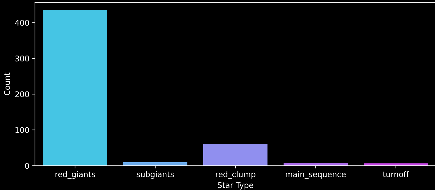
APOGEE DR17 Field: [311-06] Count plot of Star Type
