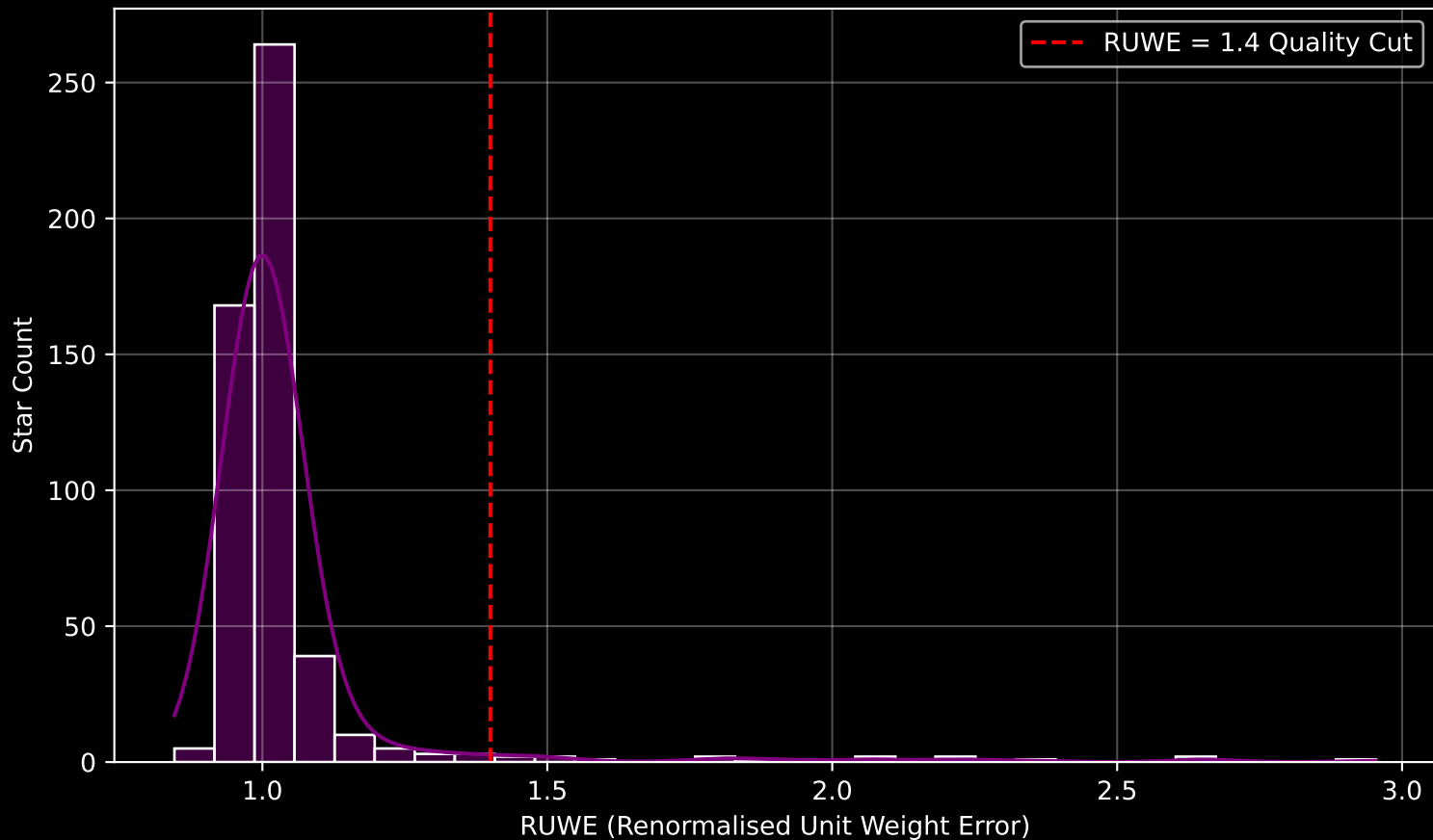
GAPOGEE DR17 Field [311-06] RUWE Distribution (n= 514)
